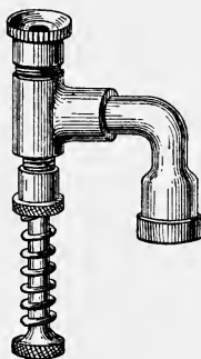
FIG. 48 VERMOREL TYPE OF NOZZLE
